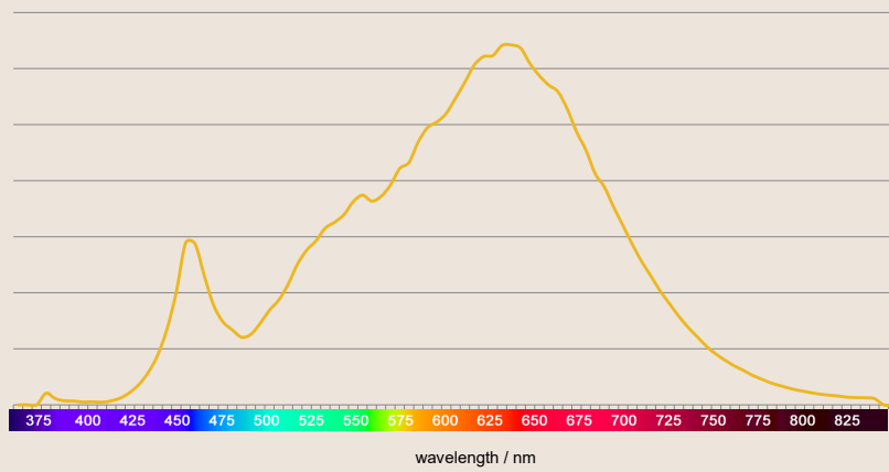
SPECTRAL POWER DISTRIBUTION OF LEDON 10W DOWNLIGHT
