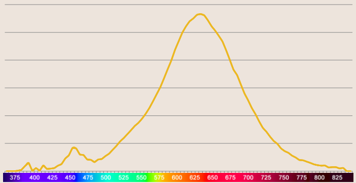
SPECTRAL POWER DISTRIBUTION OF LEDON 10W G120 Dual Color 2000K
