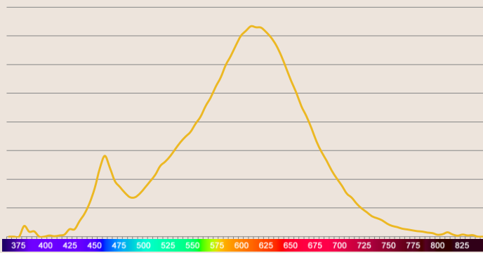
SPECTRAL POWER DISTRIBUTION OF LEDON 10W G120 Dual Color 2700K
